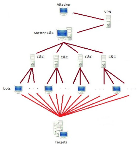
Fig. 1. A scheme of a DDoS Botnet attack
